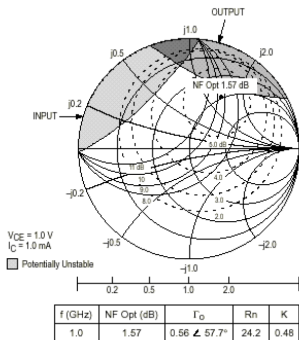
Fig. 19 Constant Gain & Noise Figure Coutours
