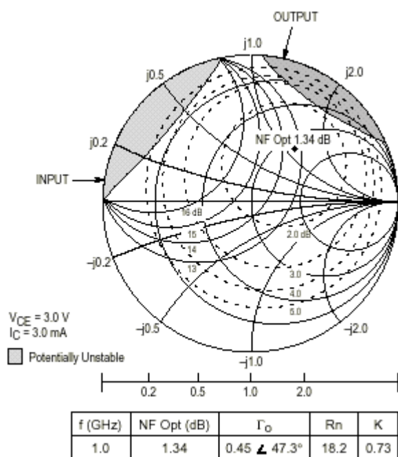
Fig. 21 Constant Gain & Noise Figure Coutours
