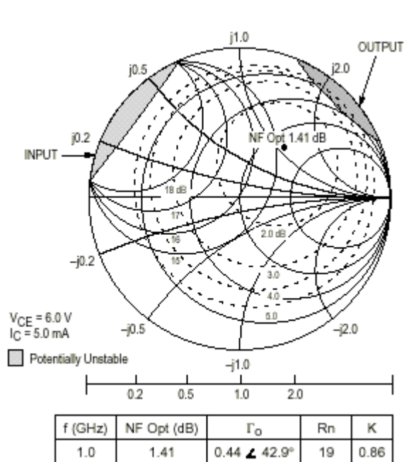
Fig. 22 Constant Gain & Noise Figure Coutours
